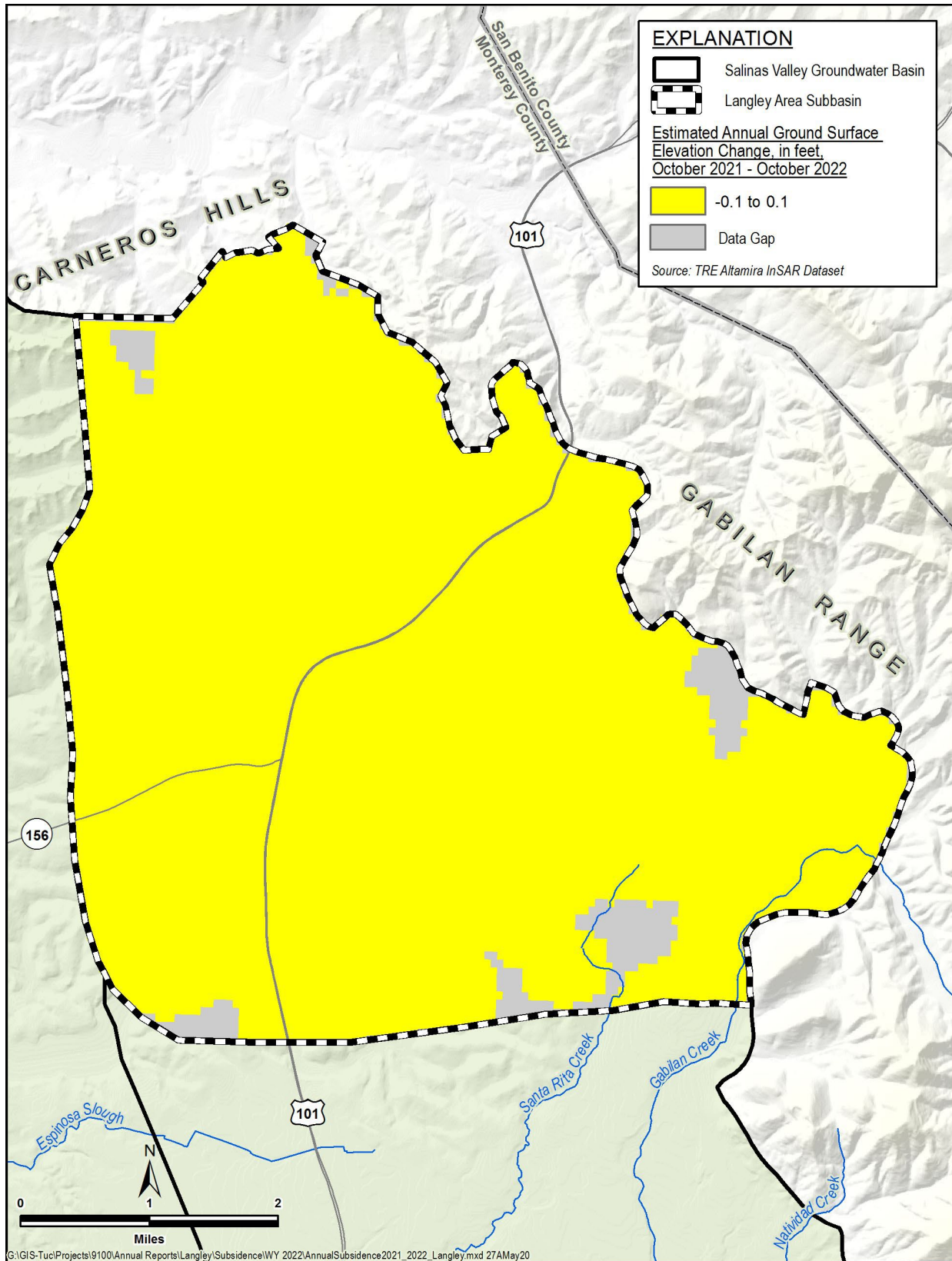
Figure 12. Annual Subsidence
