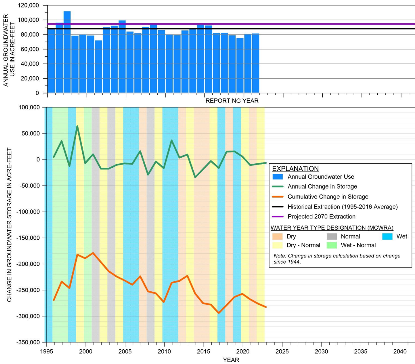
Figure 14. Groundwater Use and Annual and Cumulative Change in Groundwater Storage
